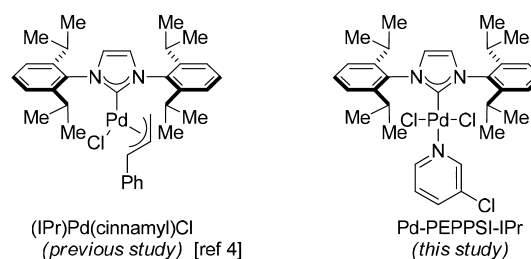
Figure 2. Highly active Pd(II)-NHC precatalysts in the Suzuki–Miyaura cross-coupling of amides.
